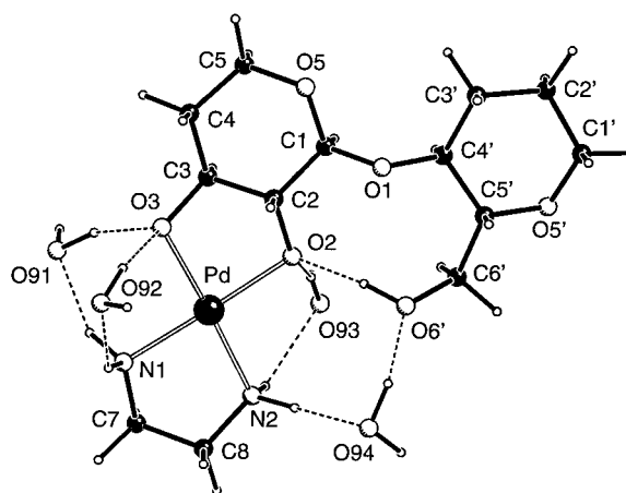
Figure 6. The minimum-energy structure of 4 ·4H 2 O. Selected distances [pm] and angles [°] (see also Tables 5 and 6): C1–C2 153.5, C2–C3 152.5, C3–C4 152.8, C4–C5 153.5, C1–O1 139.4, C1–O5 143.8, C2–O2 142.9, C3–O3 142.9, C5–O5 143.7, C4'–O1 143.8, C4'–C5' 154.0, C5'–C6' 153.7, C6'–O6' 143.0; N1–Pd–N2 84.0, O2–Pd–O3 85.4, C1–O1–C4' 118.7; O2–C2–C3–O3 57.8.
